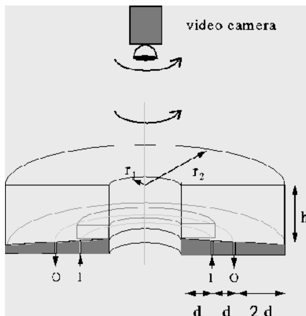
Fig. 2. Rotating annulus.
